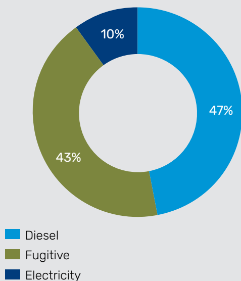
Relative Greenhouse Gas Emissions by Source
